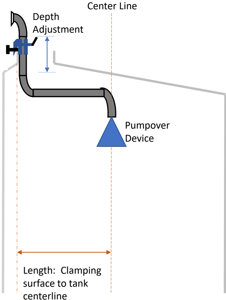
Outside Mount
