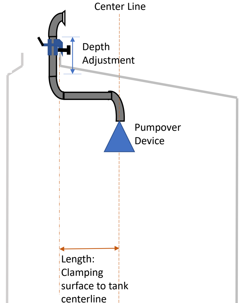
Inside Mount
